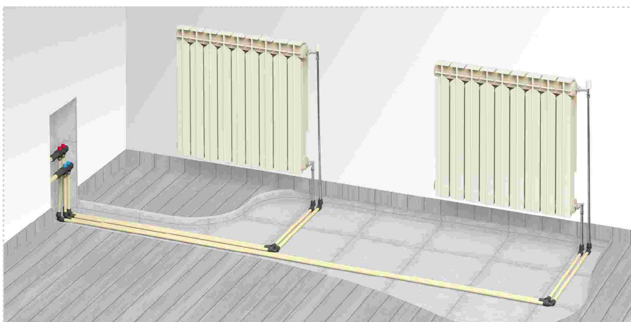
Connection to radiator for manifolds
